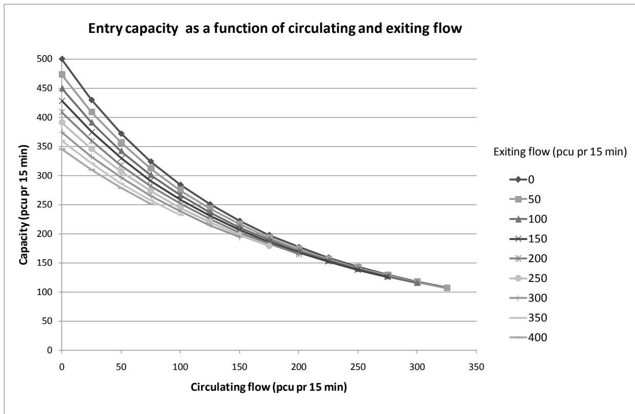
FIGURE 7. Capacity of entry lane at different circulating/exiting flow levels.
